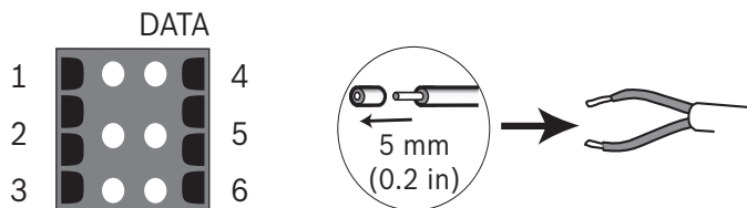
Figure 5.9 Data connector pins
